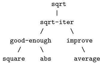
Figure 1.2: Procedural decomposition of the sqrt program.
