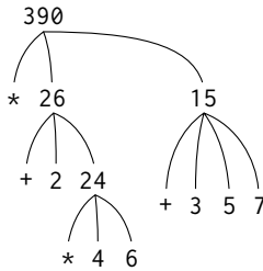
Figure 1.1: Tree representation, showing the value of each subcombination.
