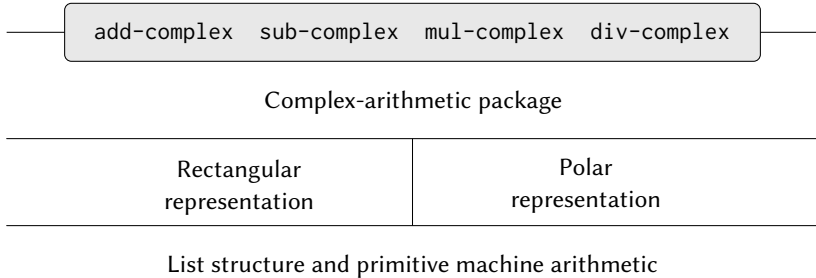
Figure 2.19: Data-abstraction barriers in the complex-number system.
